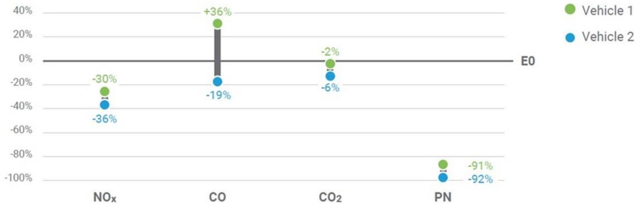
Emissions performance of E85 compared to E0 in two flex-fuel vehicles (RDE)
